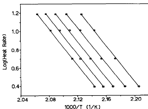
Fig. 3. Flynn and Wall plot of Fe(CO) 4 (dppf).
