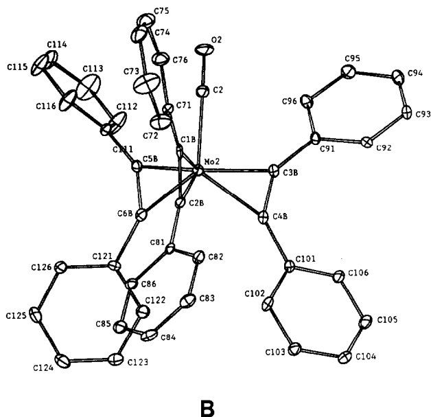
Fig. 1. Perspective view of the \text{Mo}(\text{CO})(\text{PhC}\equiv\text{CPh})_3 showing the atom-numbering scheme for two crystallographically independent molecules A and B, determined in the asymmetric unit. Hydrogen atoms have been omitted for clarity.
