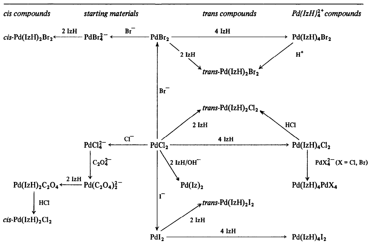
Scheme 2. Synthetic procedures for the several palladium compounds.
