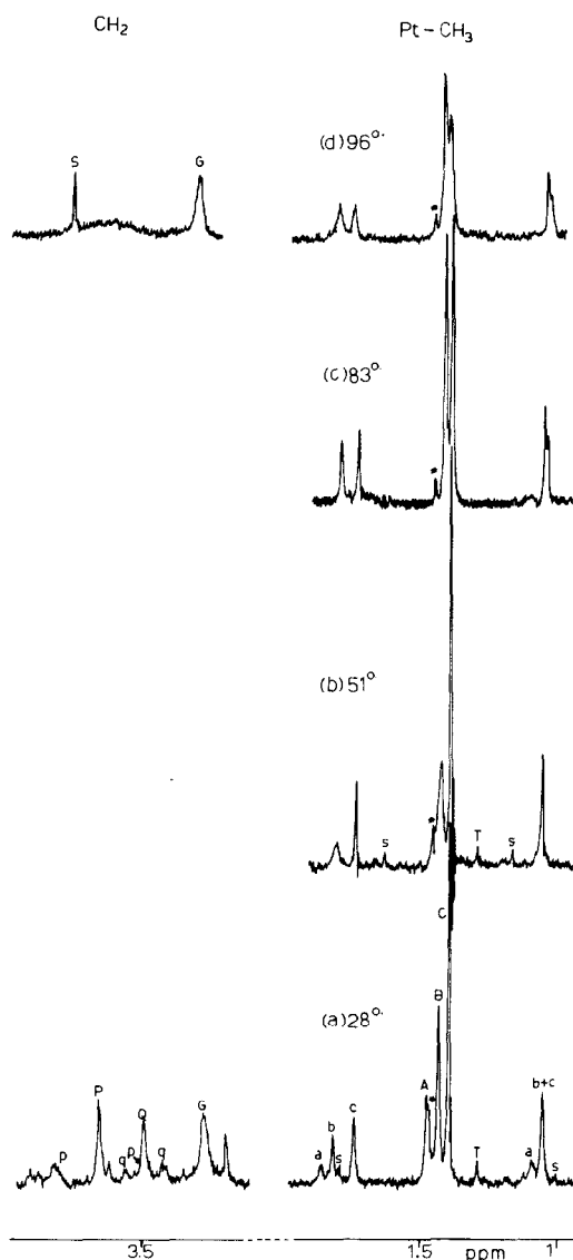
Fig. 1. Variable-temperature 100 MHz {}^1\text{H} n.m.r. spectra of \text{PtMe}_2\text{Br}(\text{gly})_2 ((36a) + (37a)) in \text{D}_2\text{O} . T, \text{PtMe}_2\text{Br}(\text{gly})_3^{2-} (38a); G, free glycinate; s spinning side band ( \text{Pt}-\text{CH}_3 ), S spinning side band ( \text{H}_2\text{O} ), * impurity. For other labels, see text.
