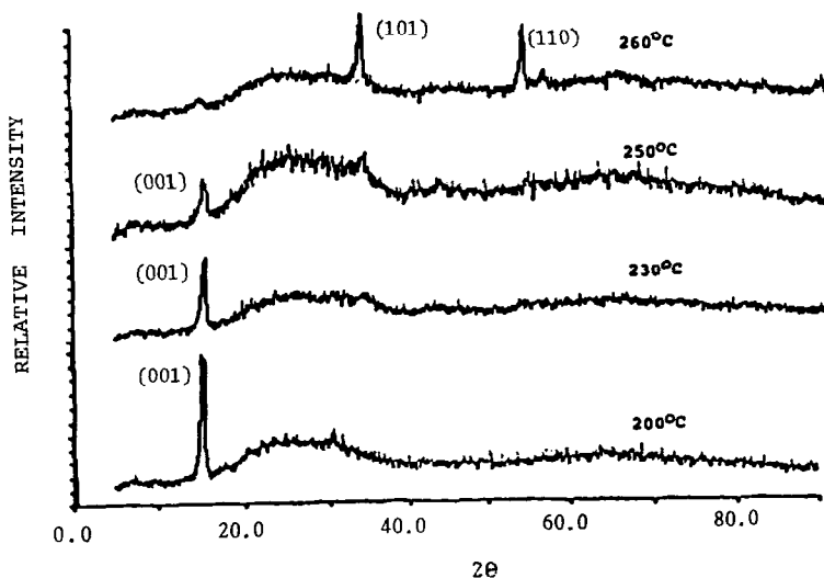
FIG. 2. XRD patterns of \text{TiS}_2 thin films prepared at different deposition temperatures.
