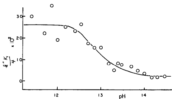
Fig. 10. Plot of rate constant k''K_1/4 against pH showing ionization of an intermediate near pH = 13.
