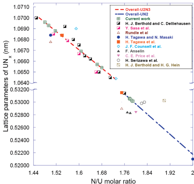
Figure 6. Change in the lattice parameter of the \text{UN}_2/\alpha\text{-U}_2\text{N}_3 system with respect to the N/U molar ratio.
