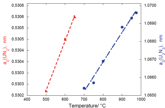
Figure 2. Lattice parameters of \text{UN}_2 and \alpha\text{-U}_2\text{N}_3 as a function of the temperature used for decomposition.
