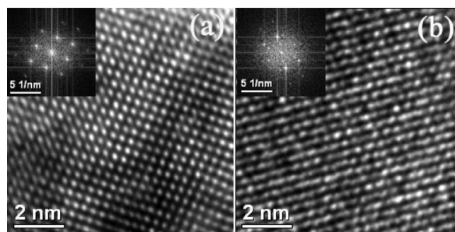
Figure 5. HRTEM images of \text{UN}_2 (a) and \text{U}_2\text{N}_3 (b). Insets are the corresponding FFT micrographs of each HRTEM image.
