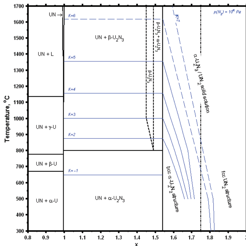
Figure 1. Equilibrium phase diagram of the pure \text{UN}_x system. 23
