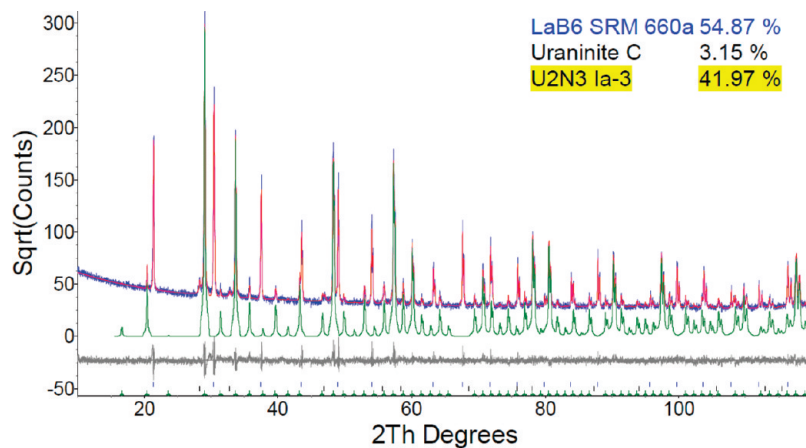
Figure 12. XRD powder refinement of \text{U}_2\text{N}_3 sample after heating it at 1100^\circ\text{C} for 30 min under \text{N}_2 -8% \text{H}_2 . The \text{U}_2\text{N}_3 calculated pattern is highlighted.
