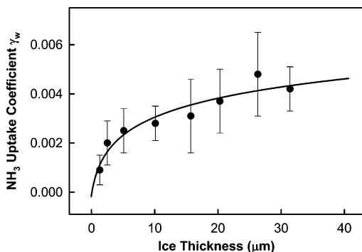
Figure 3. Plot of the initial uptake coefficient of NH 3 , \gamma_w , on the ice as a function of the ice-film thickness, at 190 K. The total pressure in the reactor was 1.000 \pm 0.003 torr, P_{\text{NH}_3} = (2.0 \pm 0.3) \times 10^{-6} torr. The solid curve is a nonlinear least-squares fit to the data using eq 3 and an empirical correlation N_L = a + b \log(h + c) , where parameters a , b , and c were fitted to be a = 0.22 , b = 3.4 , and c = 0.76 ( h = 1.3 – 31.4 \mu\text{m} ). The plot shows that \gamma_w increases from 9.0 \times 10^{-4} to 4.2 \times 10^{-3} as the ice-film thickness increases. The \gamma_t value was determined to be (3.4 \pm 1.5) \times 10^{-4} .
