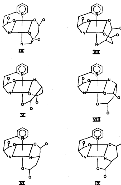
Figure 4. Isomers of [\text{Co}(\text{L-Pyala})(\text{L-Asp})] : IV, trans ( \text{O}_5 ), cis ( \text{N}_3 ); V, cis ( \text{O}_5 ), trans ( \text{N}_3 ); VI, L-fac . Isomers of [\text{Co}(\text{L-Pyala})(\text{D-Asp})] : VII, mer-cis ( \text{O}_5 ), cis ( \text{N}_3 ); VIII, trans ( \text{O}_5 ), trans ( \text{N}_3 ); IX, D-fac .
