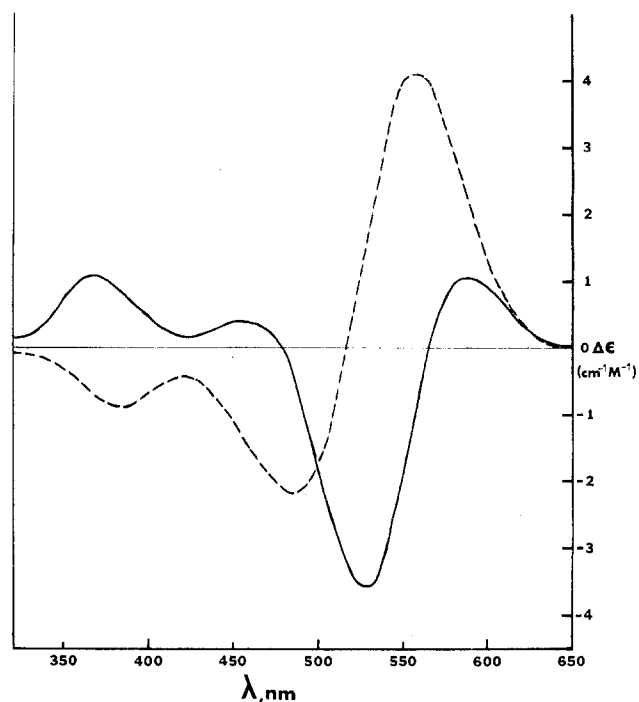
Figure 7. Circular dichroism of IV (—) and VI (---).
