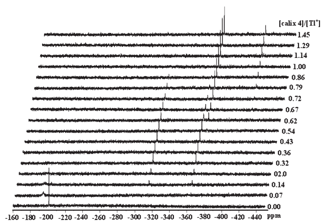
Figure 5. Thallium-203 NMR spectra of calix 4 at various ligand/ \text{TI}^+ molar ratios in \text{CD}_3\text{CN}/\text{CDCl}_3 (4:1 v/v) at 298 K.
