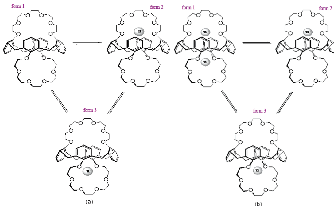
Scheme 2. Multisite Exchange Equilibria between Calix 2 and Thallium(I) Ion: (a) \text{Ti}^+/\text{Calix } \mathbf{2} Molar Ratio \leq 1 and (b) \text{Ti}^+/\text{Calix } \mathbf{2} Molar Ratio \geq 1
