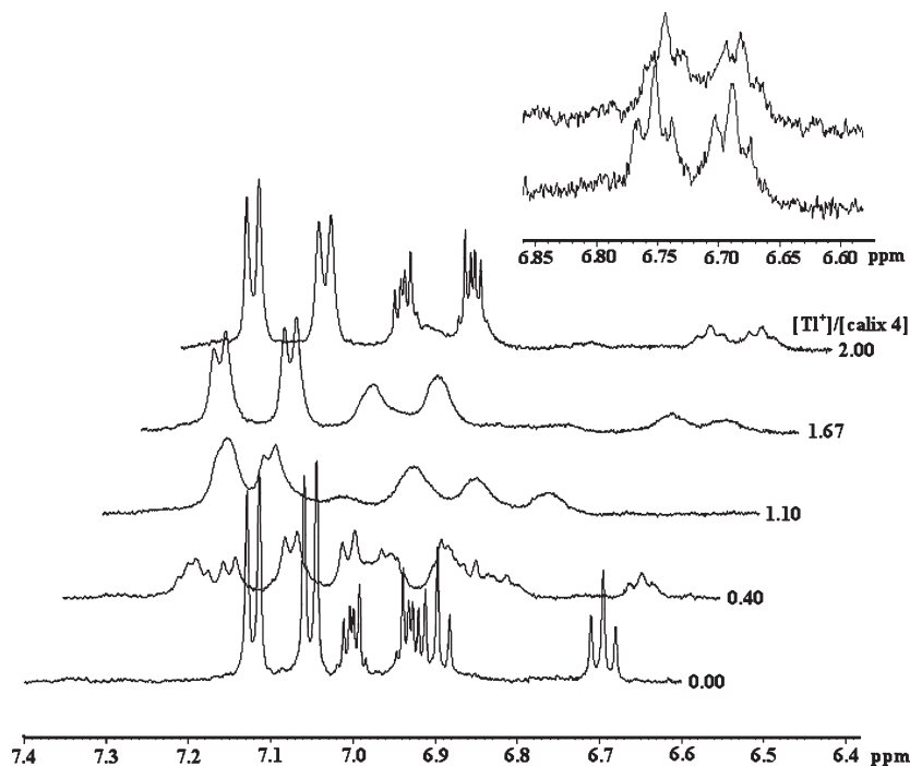
Figure 6. Proton NMR spectra of the aromatic region of calix 4 at various \text{TI}^+ /ligand molar ratios in \text{CD}_3\text{CN}/\text{CDCl}_3 (4:1 v/v) at 298 K. Inset shows the ^1\text{H} NMR spectrum of the p -H of the aryl region of calix 4 at a \text{TI}^+ /ligand molar ratio of 3.0: (top) ^{203}\text{Tl} decoupled NMR; (bottom) ^1\text{H} NMR ^{203}\text{Tl} coupled for comparison.
