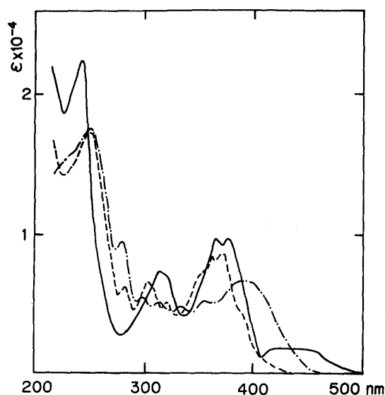
Fig. 2. UV Spectra of Compounds I and VI —, I in EtOH + HCl; ----, VI in EtOH; -----, VI in EtOH + HCl.
