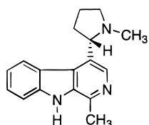
(–)-(S)-Brevicolline ( 1 )
