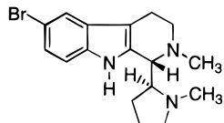
Woodinine ( 2 )
