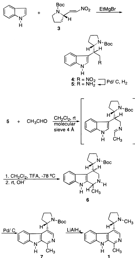
Scheme 1
