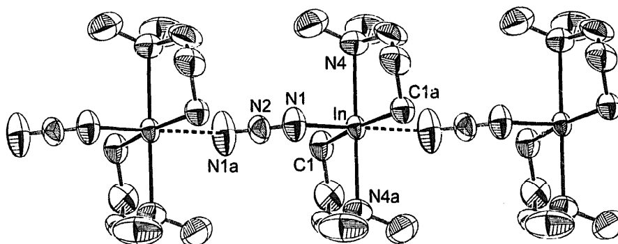
Fig. 3. Molecular structure of 3 in the solid state (ORTEP-plot with 50% probability thermal ellipsoids). Selected distances (pm) and angles (°): In–N1 252.6(2), In–N4 249.6(2), In–C1 214.8(2), N1–N2 116.5(2), N1–In–N4 88.94(8), N1–In–N4a 91.06(8), N1–In–C1 91.11(8), N1–In–C1a 88.89(8), C1–In–C1a 180.00, N4–In–N4a 180.00, N4–In–C1 80.12(8), N4a–In–C1 99.88(8), N1–N2–N1a 180.0, In–N1–N2 119.44(14).
