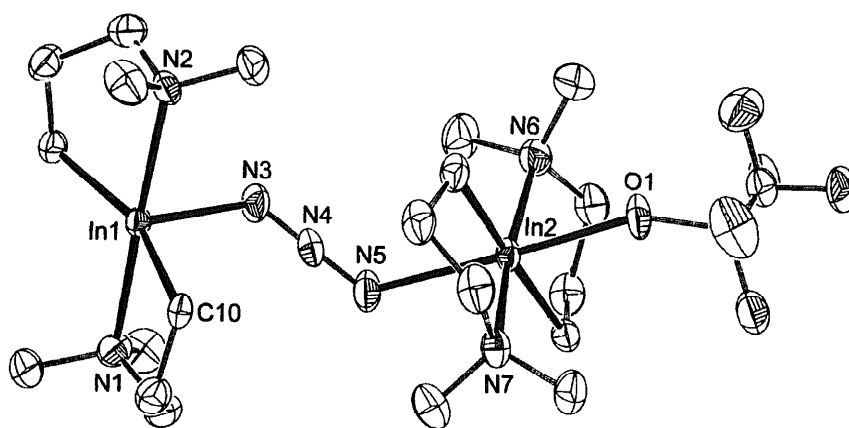
Fig. 2. Molecular structure of 2 in the solid state (ORTEP-plot with 50% probability thermal ellipsoids). Selected distances (pm) and angles (°): In1–N1 248.9(3), In1–N2 248.8(3), In1–N3 230.9(3), In1–C5 214.9(4), In1–C10 215.0(3), N3–N4 118.4(4), N4–N5 116.6(4), In2–N5 256.4(3), In2–N6 249.8(3), In2–N7 249.9(3), In2–C15 214.5(4), In2–C20 214.3(4), In2–O1 247.3(2), N1–In1–N2 173.84(10), N1–In1–N3 86.90(11), N2–In1–N3 88.37(11), N3–In1–C5 100.76(14), N3–In1–C10 100.79(15), C5–In1–C10 158.15(14), In1–N3–N4 126.3(3), N3–N4–N5 177.7(4), N4–N5–In2 123.2(2), N5–In2–N6 93.84(11), N5–In2–N7 92.64(11), N5–In2–O1 175.49(9), N6–In2–N7 173.49(10), N6–In2–C15 79.92(13), N6–In2–C20 99.14(14), N7–In2–C15 100.38(13), N7–In2–C20 80.41(14).
