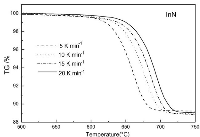
Fig. 2. The TG curves of InN in argon at heating rates of 5, 10, 15, 20 K min -1 .
