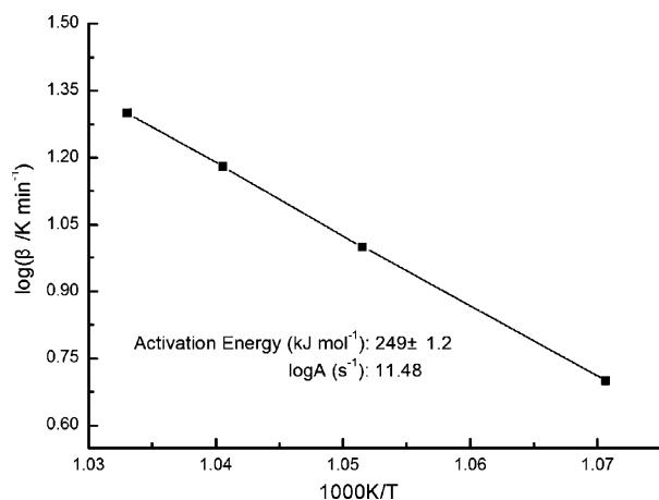
Fig. 4. The activation energy and log A obtained by the ASTM698 method for the thermal decomposition of InN in argon.
