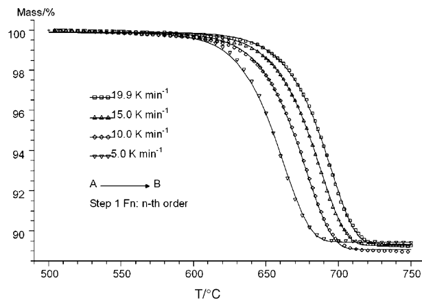
Fig. 7. The best fit of TG measurements for the decomposition of InN, simulated with reaction type F1 for the heating rates 5, 10, 15 and 20 K min -1 . The signs represent the measured data. The solid lines are the fitted curves.
