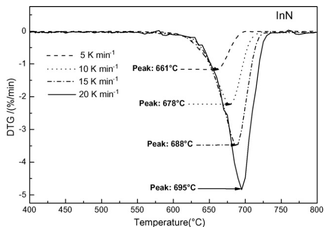
Fig. 3. The DTG curves of InN at heating rates of 5, 10, 15, 20 K min -1 .
