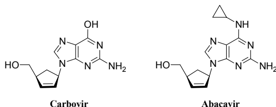
Figure 1. The structures of carbovir and abacavir
