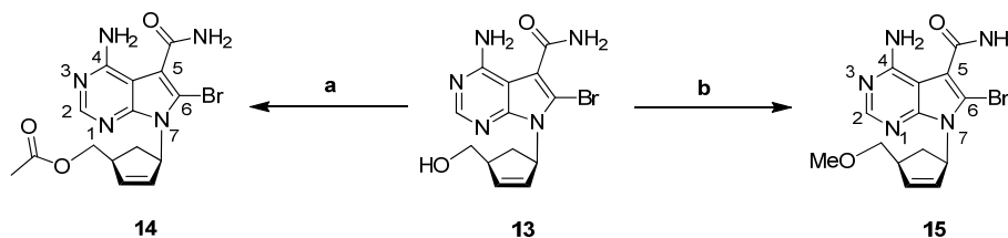
Scheme 5. Synthesis of compound 14 and 15 . Reagents and conditions: (a) Ac 2 O, pyridine, DMAP, DMSO, rt, 6 h, 90%; (b) Me 2 SO 4 , NaH, DMSO, rt, 1 h, 75%.
