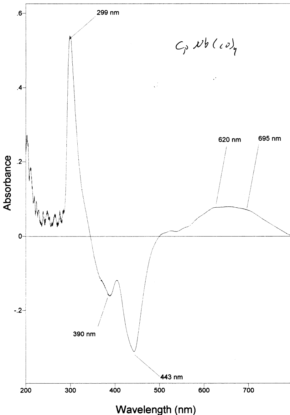
Fig. 9. Difference electronic absorption spectrum of (\eta^5\text{-C}_5\text{H}_5)\text{Nb(CO)}_4 isolated in a Nujol matrix. The difference was taken between the final photolysis 60 min irradiation at 480 < \lambda < 620 nm and 25 min irradiation at 340 < \lambda < 420 nm) and the starting material.
