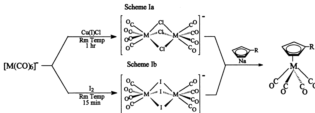
Scheme I. Synthesis of ring-substituted derivatives using [M(CO)_6]^- .
