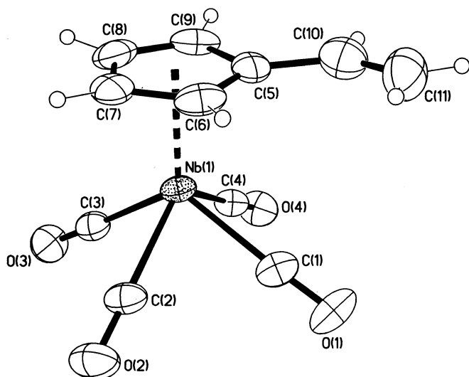
Fig. 2. Molecular structure of (\eta^5\text{-C}_5\text{H}_4\text{CH=CH}_2)\text{Nb(CO)}_4 .
