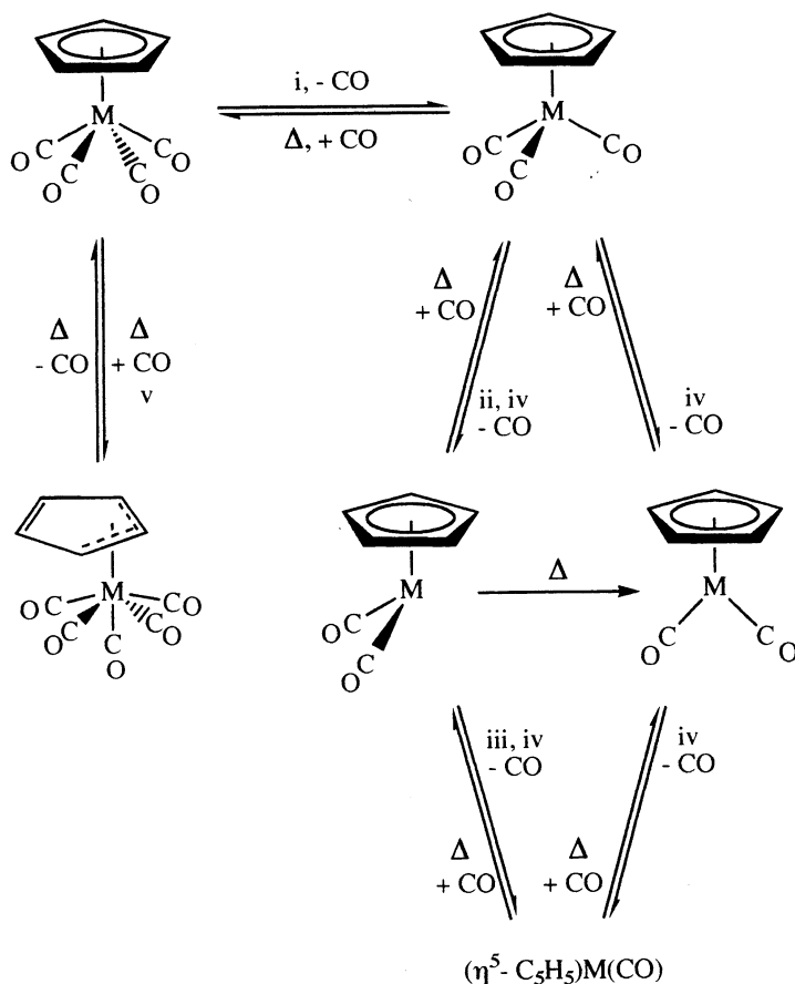
Scheme III. (i) UV–vis irradiation 222 < \lambda < 620 nm; (ii) UV irradiation 340 < \lambda < 420 nm, M = Nb , or (\eta^5-C_9H_7)Ta(CO)_4 ; (iii) UV irradiation 340 < \lambda < 420 nm, M = Nb , or (\eta^5-C_5H_5)Nb(CO)_4 or (\eta^5-C_9H_7)Ta(CO)_4 ; (iv) UV irradiation 270 < \lambda < 290 nm for (\eta^5-C_5H_5)Ta(CO)_4 or \lambda > 285 nm for (\eta^5-C_9H_7)Ta(CO)_4 ; (v) M = Ta .
