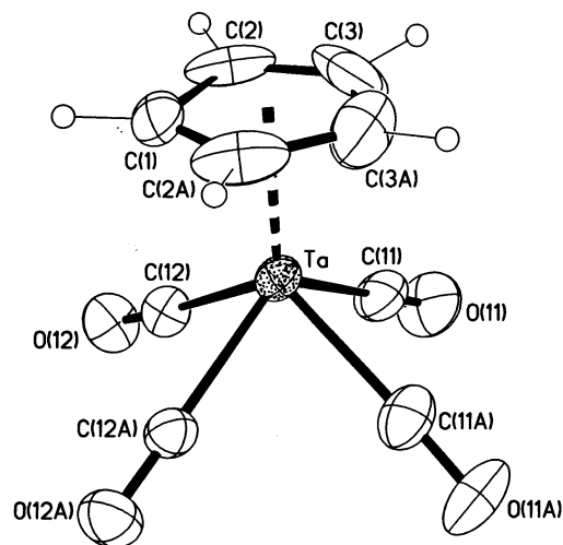
Fig. 4. Molecular structure of (\eta^5\text{-C}_5\text{H}_5)\text{Ta(CO)}_4 .
