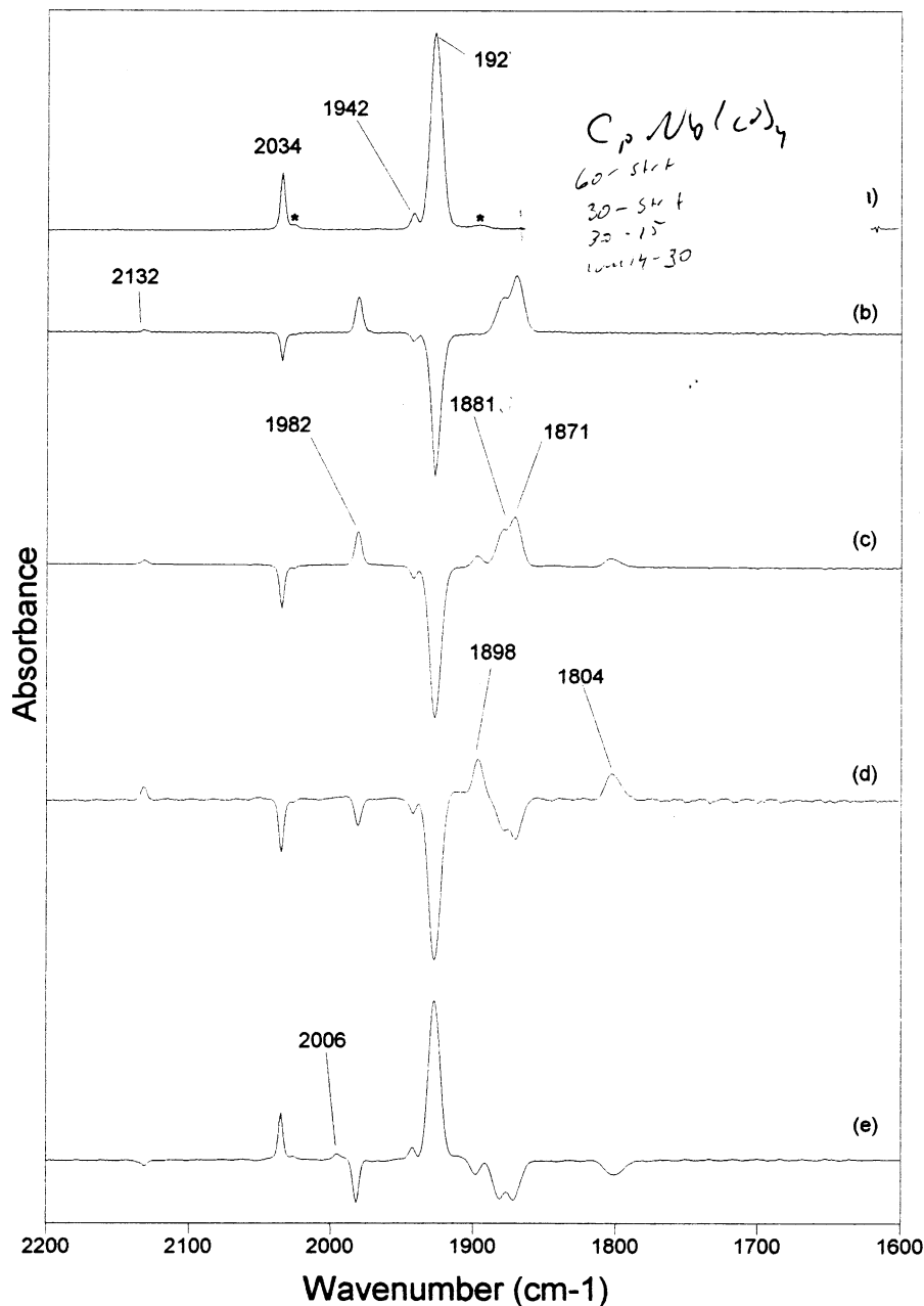
Fig. 7. IR spectra with ( \eta^5 -C 5 H 5 )Nb(CO) 4 isolated in a Nujol matrix: (a) starting material, (b) subtraction spectrum, 60 min irradiation at 480 < \lambda < 620 nm minus starting material, (c) subtraction spectrum, 30 min irradiation at 340 < \lambda < 420 nm minus starting material, (d) subtraction spectrum, difference between two 15 min periods of irradiation at 340 < \lambda < 420 nm, (e) subtraction spectrum, anneal to 133 K minus final photolysis. * Arise from ( \eta^5 -C 5 H 5 )Nb(CO) 3 ( 13 CO) present in natural abundance.
