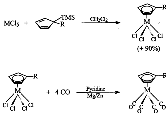
Scheme II. High yield synthesis of (\eta^5-C_5H_5)M(CO)_4 from (\eta^5-C_5H_5)MCl_4 .
