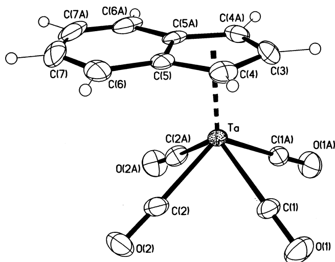
Fig. 3. Molecular structure of (\eta^5\text{-C}_9\text{H}_7)\text{Ta(CO)}_4 .
