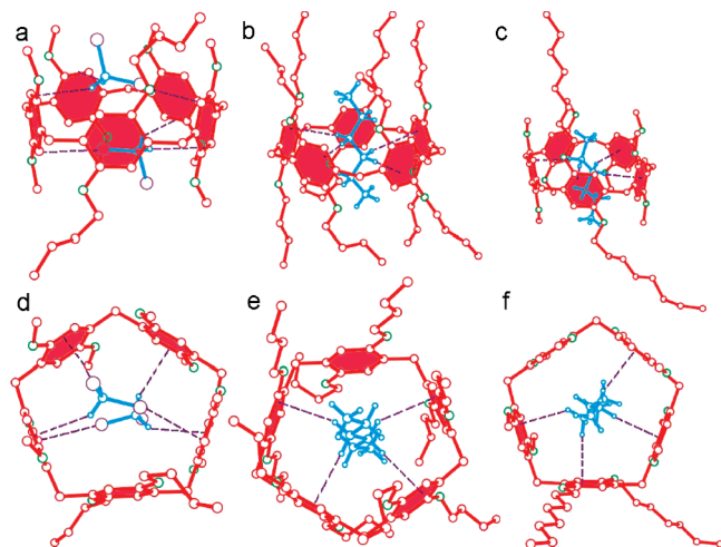
Figure 2. Views of the crystal structures of 1 ⊃(CH 2 Cl 2 ) 2 (a, d), 5 ⊃n-C 6 H 14 (b, e), and 3 ⊃n-C 6 H 14 (c, f). Hydrogens on 1 , 3 , and 5 were omitted for clarity; 1 , 3 , and 5 are red, oxygen atoms are green, chlorine atoms are magenta, and dichloromethane and n-hexane molecules are blue. The purple dotted lines indicate C-H...π interactions and halogen bonds.
