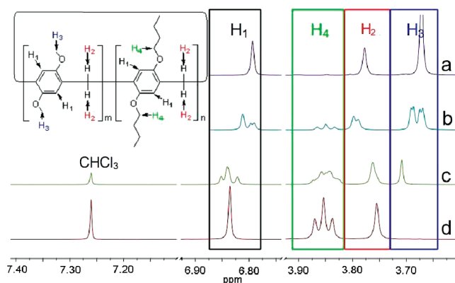
Figure 1. Partial ^1\text{H} NMR spectra (400 MHz, \text{CDCl}_3 , 20 °C) of (a) homopillar[5]arene 4 ( m = 5 , n = 0 ); (b) copillar[5]arene 1 ( m = 4 , n = 1 ); (c) copillar[5]arene 2 ( m = 1 , n = 4 ); (d) homopillar[5]arene 5 ( m = 0 , n = 5 ).
