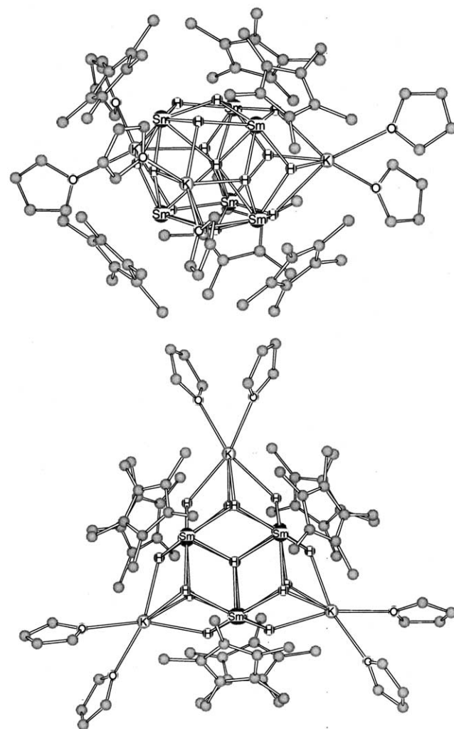
Fig. 1. X-ray structure of 26 . Top: a general view. Bottom: a view along the threefold axis. The Sm–C 5 Me 5 bonds are omitted for clarity.
