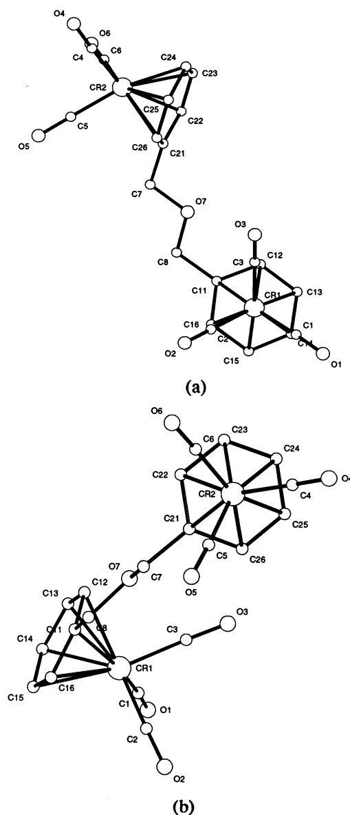
Fig. 2. (a) The crystal structure of [Cr(CO) 3 (C 6 H 5 CH 2 OCH 2 C 6 H 5 )Cr(CO) 3 ] ( 2 ), (view down Cr1-centroid axis). (b) [Cr(CO) 3 (C 6 H 5 CH 2 OCH 2 C 6 H 5 )Cr(CO) 3 ] ( 2 ), (view down Cr2-centroid axis).
