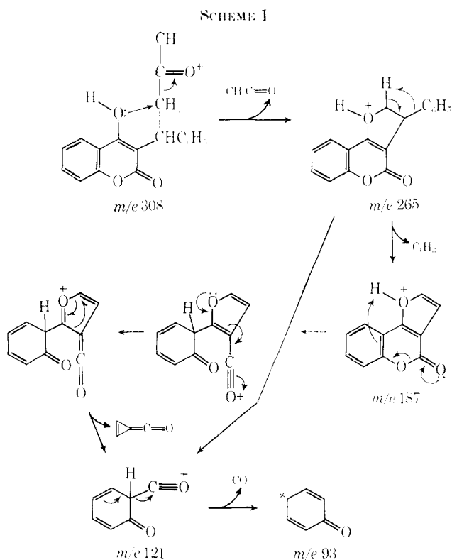
Figure 2.—Mass spectrum of 3 ; ( \leftrightarrow ) indicates the fragmentation route for Scheme I, ( \leftrightarrow ) indicates the fragmentation route for Scheme III.
