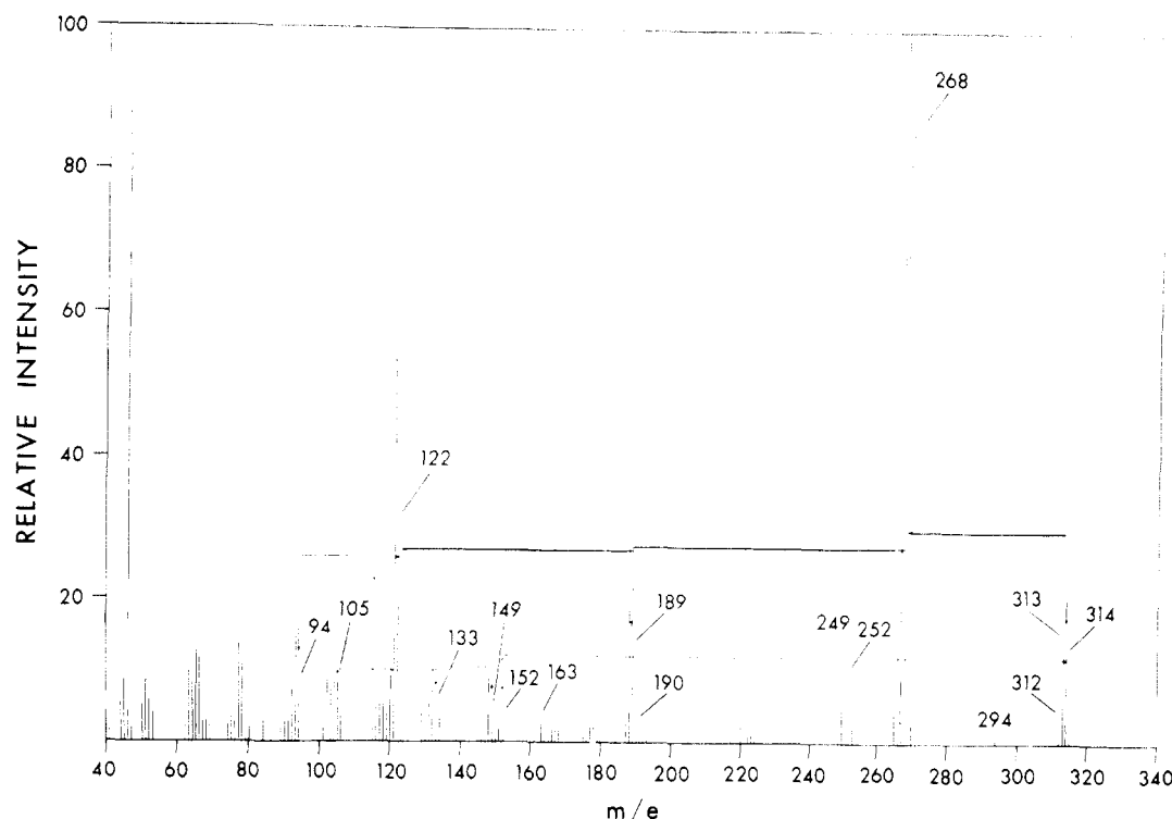
Figure 2.—Mass spectrum of 3 ; ( \leftrightarrow ) indicates the fragmentation route for Scheme I, ( \leftrightarrow ) indicates the fragmentation route for Scheme III.
