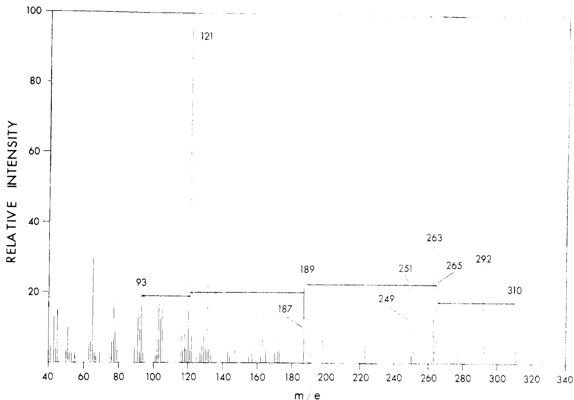
Figure 8.—Mass spectrum of 1h ; ( \leftrightarrow ) indicates the fragmentation route analogous to that shown in Scheme I.
