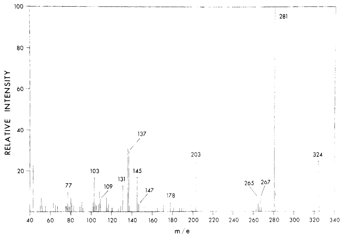
Figure 6.—Mass spectrum of 1e .
