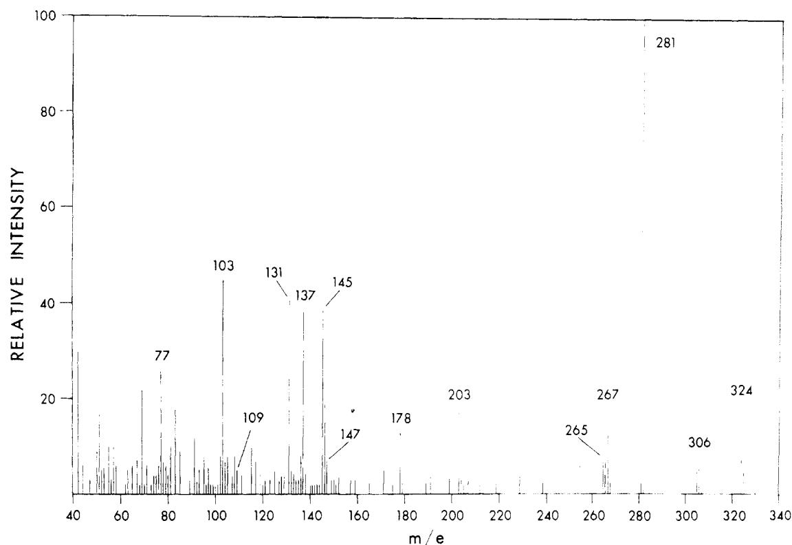
Figure 5.—Mass spectrum of 1b .
