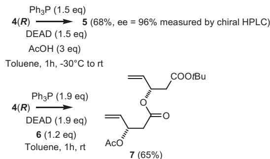
Scheme 4. Mitsunobu reactions on hydroxyester 4(R) ( 1 ).
