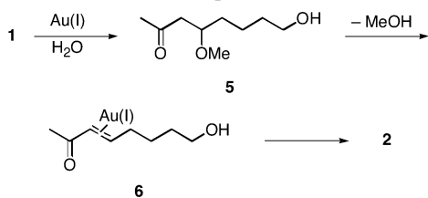
Scheme 2. Proposed Mechanism
