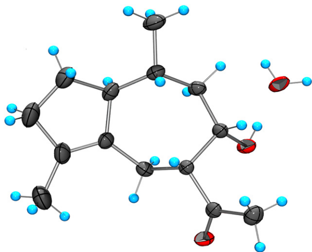
Figure 1. ORTEP diagram of the hydroxy ketone 26a .
