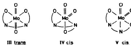
Fig. 6. Cis and trans structures for dioxo[bis(salicylaldehyde-polymethylenediiminato)molybdenum(VI)].
