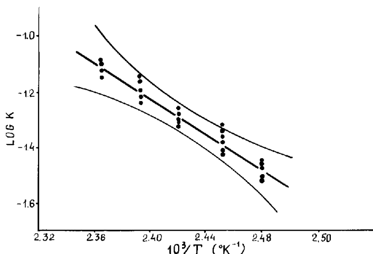
Fig. 4. Arrhenius dependence of thermal K_3CrO_8 decomposition rate constants.
