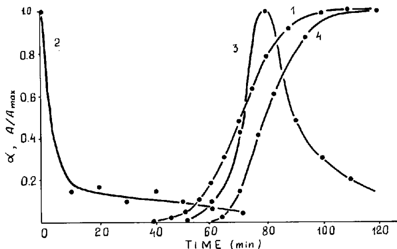
Fig. 10. Variation of the number of different paramagnetic centres (relative units): 1, kinetic curve of \text{K}_3\text{CrO}_8 thermolysis at 403 K; 2, \text{CrO}_8^{3-} ; 3, matrix-isolated \text{CrO}_8^{3-} ; 4, ion-radicals \text{O}_2^- .
