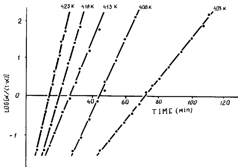
Fig. 3. Linearized form of kinetic K_3CrO_8 thermolysis curves.
