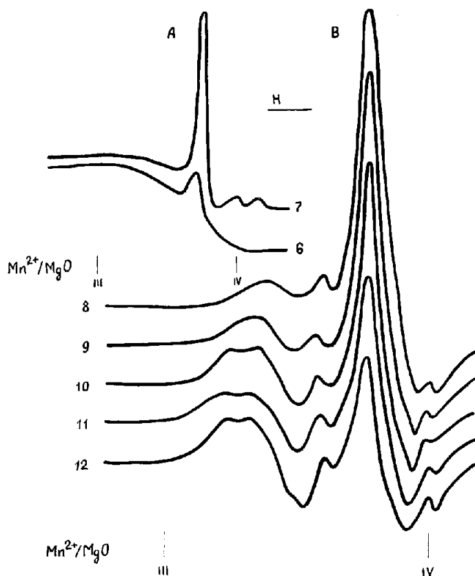
Fig. 11. ESR spectra of \text{K}_3\text{CrO}_8 in the intensive decomposition period (B signals are twice magnified compared to A signals); 6, 7, 8, 9, 10, 11 and 12 represent 60, 70, 80, 90, 100, 110 and 120 min of heating, respectively.
