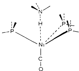
Fig. 1. Sketch drawing of the product of the reaction between [(\text{np}_3)\text{NiH}]^+ and CO.
