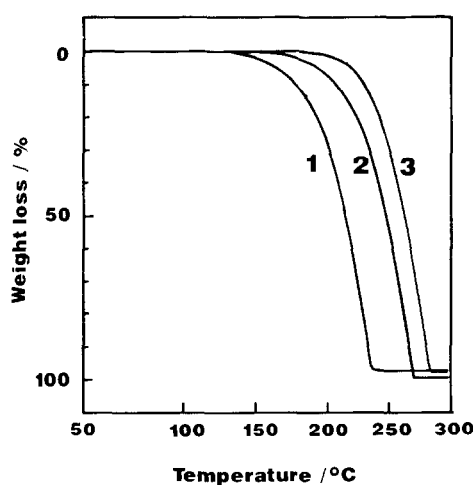
Fig. 1. Thermograms of thallium, ytterbium and neodymium chelates with 2,2,6,6-tetramethyl-3,5-heptanedione. 1: Tl(thd); 2: Yb(thd) 3 ; 3: Nd 2 (thd) 6 .
