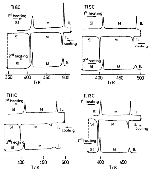
Fig. 2. Thermograms (volatile pans) showing the fusion and clearing transitions of thallium(I) n -alkanoates (Tl n C). M, mesophase; IL, isotropic liquid.
