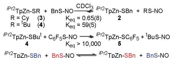
Scheme 3. Transnitrosation Equilibria at Zinc Thiolates in CDCl 3
