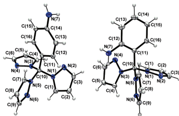
FIGURE 2. ORTEP drawing (50% ellipsoids) with atom labeling of p - (left) and o -H 2 NC 6 H 4 C(pz) 3 (right).
