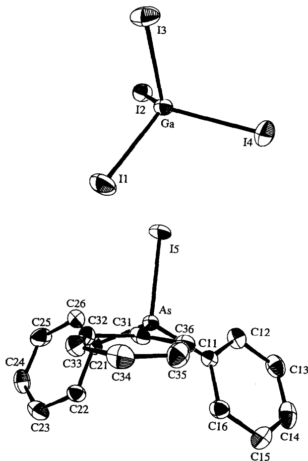
Fig. 2. View (ORTEP) of \text{Ph}_3\text{AsI}^+ and \text{GaI}_4^- . Important bond distances (Å): Ga–I 2.547(1) (average), As–I 2.485(1), As–C 1.914(8) (average).
