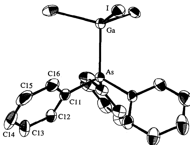
Fig. 1. View (ORTEP) of \text{Ph}_3\text{AsGaI}_3 . Important bond distances (Å) and angles ( ^\circ ): As1–Ga1 2.489(2), Ga1–I1 2.509(1), As1–C1 1.919(2), I1–Ga1–I1 115.11(1), C1–As–C1 105.49(8) torsion angle I–Ga–As–C1 81.6(1).
