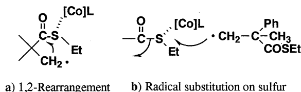
Figure 2. Possible mechanism of the involvement of cobaloxime(II) in the radical processes.
