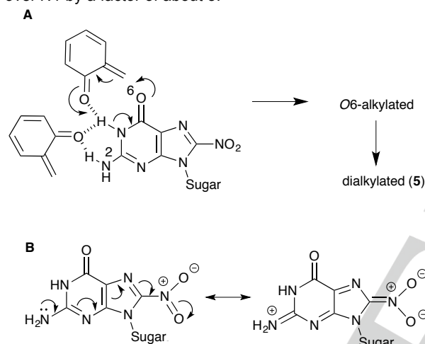
Scheme 2. Panel A shows O6 versus N2 hydrogen bond-directed alkylation, resulting in initial alkylation at the presumably more reactive O6 position and subsequent alkylation at N2, to give dialkylated 5 . Panel B shows reduced nucleophilicity of N2 because of conjugation through to the nitro group.
