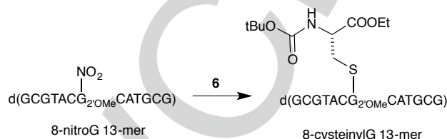
Scheme 5. Reaction of nitro-13-mer with cysteine nucleophile 6 .
