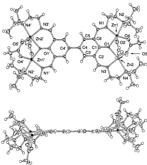
Figure 1. Top and side view of [\text{Zn}_4(\text{L})(\mu\text{-CH}_3\text{CO}_2)_4]^{2+} cation; Selected distances (Å) : \text{Zn}(1)\text{-Zn}(2) = 3.2441(9) , \text{Zn}(1)\text{-O}(1) = 2.154(4) , \text{Zn}(1)\text{-O}(2) = 1.977(4) , \text{Zn}(1)\text{-O}(4) = 1.976(4) , \text{Zn}(1)\text{-N}(1) = 2.014(5) , \text{Zn}(1)\text{-N}(2) = 2.243(5) , \text{Zn}(2)\text{-O}(1) = 2.112(4) , \text{Zn}(2)\text{-O}(3) = 1.963(4) , \text{Zn}(2)\text{-O}(5) = 1.973(4) , \text{Zn}(2)\text{-N}(3) = 2.027(5) , \text{Zn}(2)\text{-N}(4) = 2.237(5) , \text{C}(4)\text{-C}(4') = 1.512(4) , \text{C}(1)\text{-O}(1) = 1.296(7) Å.
