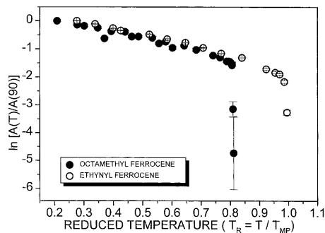
Fig. 5. The temperature dependence of the recoil-free fraction for OMF and 1 . The abscissa is the reduced temperature, T_R = T/T_{MP} , where the melting points are those of OMF and 1 , respectively. The large error bars of the highest temperature measurements reflect the very small values of the resonance effect magnitude, although in excess of 8 \times 10^6 counts per channel were acquired in the individual experiments.
