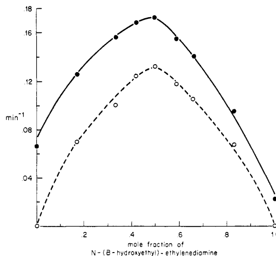
Figure 1. The change in k_e' as a function of the mole fraction of N -( \beta -hydroxyethyl)ethylenediamine: pH 7.10; 0.03 M Hepes; 0.1 M NaCl. Total concentration of \text{Zn}^{2+} plus 1 is 2.06 \times 10^{-3} M . In all runs, the p -nitrophenylpicolinate concentration is 7.78 \times 10^{-5} ; solid line, uncorrected rate constants; dashed line, rate constants corrected for free zinc ion and free 1 concentrations.
