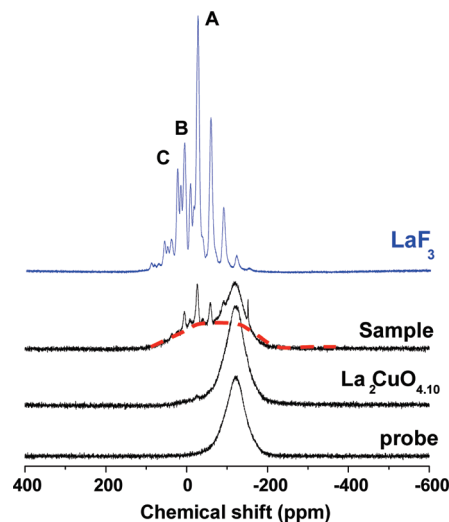
Figure 6. ^{19}\text{F} MAS NMR spectra of \text{LaF}_3 , \text{La}_2\text{CuO}_{4.10} , the fluorinated sample, and the probe ( T = 300 K).
