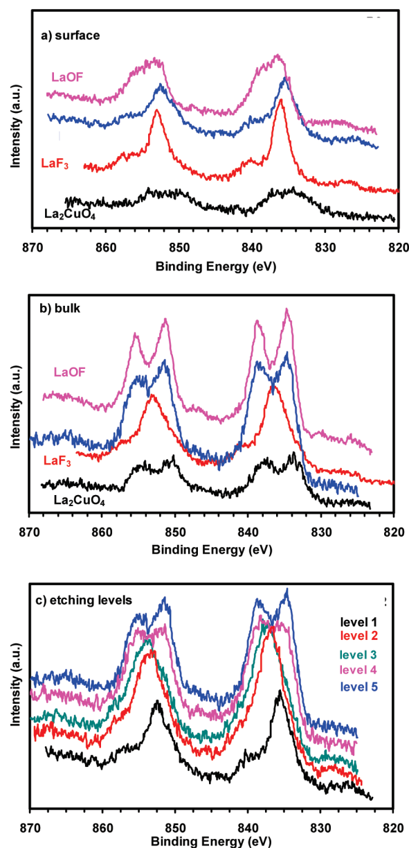
Figure 4. La3d high-resolution XPS spectra of (a) the surface of the fluorinated sample (blue), LaF 3 , LaOF, and La 2 CuO 4-01 ; (b) the bulk of the fluorinated sample (blue), LaF 3 , LaOF, and La 2 CuO 4-01 ; and (c) fluorinated sample: depth profile analysis after 0, 60, 120, 300, and 480 s etching times.
