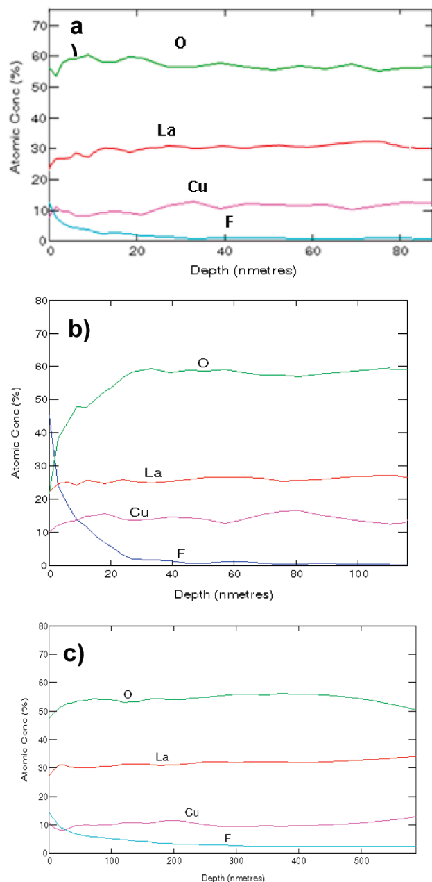
Figure 1. Auger depth profile of the elements present in the \text{La}_2\text{CuO}_{4-(\text{O},\text{F})} phases prepared (48h) at (a) 300 \mu\text{A}/\text{cm}^2 in \text{DMSO}/n\text{Bu}_4\text{NBF}_4 (0.1 M), (b) 100 \mu\text{A}/\text{cm}^2 in \text{CH}_3\text{CN}/n\text{Bu}_4\text{NF} (0.1 M), and (c) 600 \mu\text{A}/\text{cm}^2 in \text{DMF}/n\text{Bu}_4\text{NBF}_4 (0.1 M).
