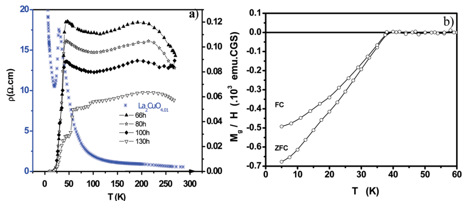
Figure 2. (a) Thermal variation of the electrical resistance of \text{La}_2\text{CuO}_{4.01} (starting material, (*)) after electrochemical treatment in \text{DMF}/n\text{Bu}_4\text{NBF}_4 ( 600 \mu\text{A cm}^{-2} ), for various times of polarization ( 66 \text{ h} \leq t_{\text{ox}} \leq 130 \text{ h} ). (b) Thermal variation of the magnetic susceptibility of the inserted sample obtained after 130 h. FC, field-cooled; ZFC, zero-field-cooled.
