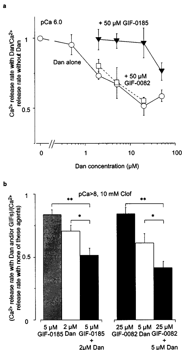
Figure 4 Different effect of GIF-0082 and GIF-0185 on \text{Ca}^{2+} release. (a) In skinned fibres, the rates of \text{Ca}^{2+} release measured with Dan (0–50 \mu\text{M} ) at pCa 6.0 under \text{Mg}^{2+} -free conditions were normalized to the control value (without Dan) obtained in the same preparation in the absence (Dan alone, mean \pm s.e.mean, n=3-6 ) or presence of 50 \mu\text{M} GIF-0082 ( n=3 ) or GIF-0185 ( n=5 ). (b) The rates of \text{Ca}^{2+} release by 10 mM Clof in the presence of Dan (2 or 5 \mu\text{M} , mean \pm s.e.mean) and/or either GIF-0185 (5 \mu\text{M} ) or GIF-0082 (25 \mu\text{M} , n=4 ) under \text{Ca}^{2+} , \text{Mg}^{2+} -free conditions (buffered with 10 mM EGTA) were normalized to the control value (without these agents) within each preparation. * P<0.05 , ** P<0.01 .
