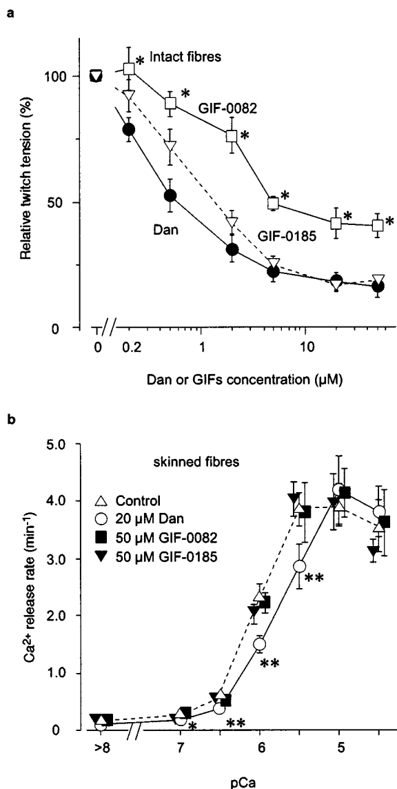
Figure 2 Effects of Dan, GIF-0082, and GIF-0185 on \text{Ca}^{2+} release. (a) In intact fibres, after treatment with dantrolene (Dan), GIF-0082, or GIF-0185 in the concentration range of 0.2–50 μM, the size of twitch contraction was compared with that before the treatment. Relative tensions were plotted against the concentrations. (mean ± s.e.mean, n=9 for Dan, n=3-6 for GIF-0082, n=3-6 for GIF-0185). * P<0.05 (Dunnett's test). (b) The rates of \text{Ca}^{2+} release were obtained in saponin-skinned fibres with 20 μM Dan ( n=5 ), 50 μM GIF-0082 ( n=3-7 ) or 50 μM GIF-0185 ( n=3-4 ) in the absence of \text{Mg}^{2+} and adenine nucleotide at pCa >8–4.5. Open triangles show the rates without these agents (control, n=11-16 ). The symbols for GIF-0082 and GIF-0185 were slightly offset horizontally for clarity (mean ± s.e.mean). * P<0.05 , ** P<0.01 (vs control). Error bars smaller than the symbols are not shown.
