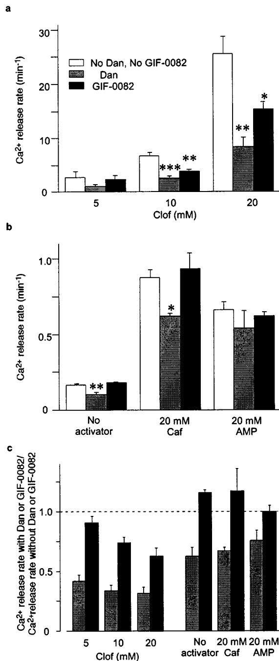
Figure 3 Effects of Dan and GIF-0082 on caffeine- and clofibric acid-induced \text{Ca}^{2+} release in skinned fibres. The rates of \text{Ca}^{2+} release with 20 μM Dan or 50 μM GIF-0082 were measured under \text{Mg}^{2+} - and \text{Ca}^{2+} -free conditions (buffered with 10 mM EGTA) with 5–20 mM clofibric acid (Clof, Figure 3a, mean ± s.e.mean, n=3-6 ) or with or without CICR activators (caffeine, Caf; AMP; Figure 3b, n=5-7 ). Note the difference in the scales. (c) The results in a and b were normalized to the control value (without Dan or GIF-0082) within each preparation. * P<0.05 , ** P<0.01 , *** P<0.001 .
