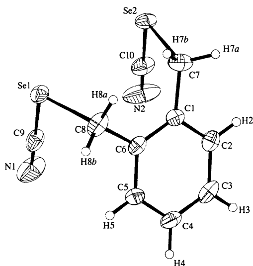
Fig. 1. SNOOPI (Davies, 1983) 30% probability displacement ellipsoid plot of C_6H_4(CH_2SeCN)_2 .
