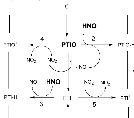
Scheme 1. Mechanism Underlying the Conversion of PTIO to PTI and PTI-H by HNO at pH 7.0 a
