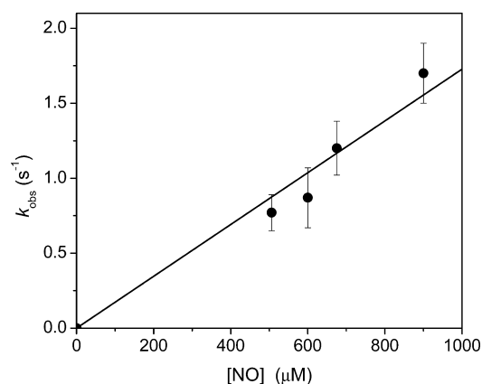
Figure 7. Dependence of the pseudo-first-order rate constant of the decay of C-PTIO-H on [NO] at pH 7.0 and 22 °C. Equal volumes of C-PTIO-H (120 \mu M, 10 mM PB, Ar-saturated) and NO (0.9–1.8 mM, 10 mM PB) were mixed using the stopped-flow apparatus, and the decay of C-PTIO-H was followed at 320 nm.
