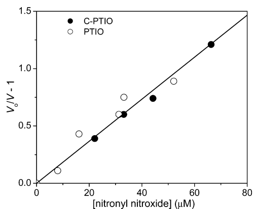
Figure 5. Effects of nitronyl nitroxide on the initial rate of MbFe II NO formation analyzed according to eq 10. The rate of MbFe II NO formation was measured at 425 nm upon exposure of 10 \mu M MbFe III OH 2 to 44 \mu M AS in aerated solutions containing 10 mM PB at pH 7.0 and 22 °C.
