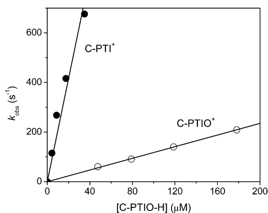
Figure 6. Dependence of the pseudo-first-order rate constants for the decays of C-PTIO + and C-PTI + on [C-PTIO-H] at pH 7 and 22 °C. Equal volumes of C-PTIO-H (9–356 \mu M) and C-PTIO + (20 \mu M) or C-PTI + (2–20 \mu M), all in 10 mM PB, were mixed using the stopped-flow apparatus, and the decay of the absorption was followed at 450 or 320 nm, respectively.
