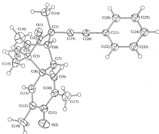
Fig. 1 X-Ray molecular structure of spirocyclohexa-2,5-dienone 16 (with atomic numbering used in the crystallographic data)
