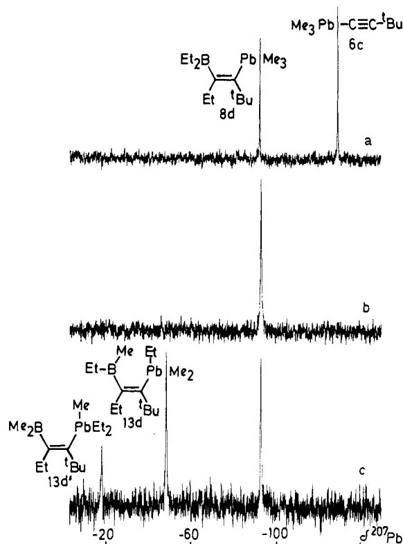
Figure 4. 62.8-MHz 207 Pb{ 1 H} NMR spectra for monitoring the formation of 8d and its rearrangement into 13d and 13d': (a) spectrum taken at -50^\circ C , after mixing 6c and 2a at -78^\circ C in CD_2Cl_2 , showing that 6c is still present; (b) spectrum taken after 10 min at -15^\circ C , showing that 6c is fully consumed and 8d is the only product; (c) spectrum taken at -15^\circ C immediately after warming the sample to 25^\circ C for 60 s, now showing a mixture of 8d, 13d, and 13d' (note that the line widths of the 207 Pb resonances are very similar, as expected for an unchanged stereochemistry at the C=C double bond). If the mixture is left at 25^\circ C for 1 h, 8d is no longer detectable and 13d and 13d' (ratio \sim 2:1 ) are the main products, together with a growing number of further unidentified products due to decomposition.
