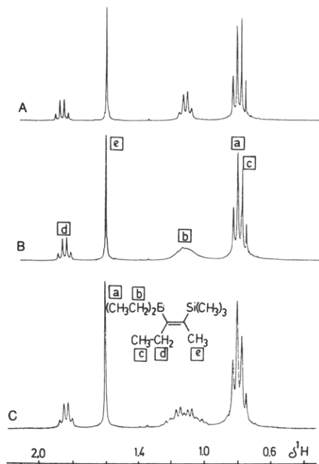
Figure 1. Part of the 300-MHz ^1\text{H} NMR spectra of ( E )-2-(trimethylsilyl)-3-(diethylboryl)-2-pentene ( 3 , L_nM = \text{Me}_3\text{Si} , R^1 = \text{Me} , R = \text{Et} ; the ^1\text{H} \text{SiMe}_3 resonance is not shown) at various temperatures: (A) -20^\circ\text{C} , corresponding to the spectrum at 25^\circ\text{C} (the rotation of the \text{Et}_2\text{B} group about the =\text{C}-\text{B} bond is fast, and the ^1\text{H} \text{BET} resonance shows the pattern for an \text{A}_2\text{M}_3 spin system); (B) -45^\circ\text{C} (the rotation of the \text{Et}_2\text{B} group about the =\text{C}-\text{B} bond is slow, indicating coalescence); (C) -70^\circ\text{C} (the pattern of an \text{ABM}_3 spin system has emerged, which upon ^1\text{H}\{^1\text{H}\} decoupling yields the coupling constant ^2J(^1\text{H}^1\text{H}) = 18 \pm 0.3 Hz; with use of the value ^2J(^1\text{H}^1\text{H}) = 18.0 Hz and the shift difference \Delta(^1\text{H}) = 20.9 Hz, \Delta G^*(-45^\circ\text{C}) = 46.5 \pm 2 kJ/mol for the barrier to rotation of the \text{Et}_2\text{B} group about the =\text{C}-\text{B} bond can be evaluated 28 ). The quality of analogous spectra for 7b ( L_nM = \text{Me}_3\text{Sn} ) and 8b ( L_nM = \text{Me}_3\text{Pb} ) is poor, owing to smaller shift differences \Delta(^1\text{H}) and broadening of all ^1\text{H} resonances at low temperature ( <-70^\circ\text{C} ).
