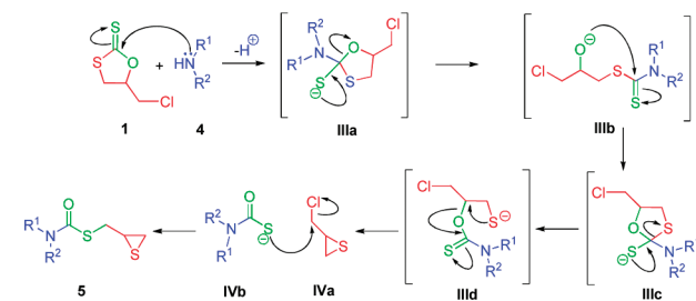
Scheme 4. Mechanistic Pathway of the Reaction of 1 with 4
