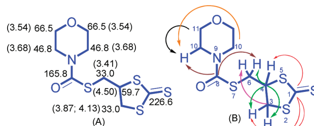
Figure 1. 1 H NMR (in parentheses) and 13 C NMR values (A) and 13 C to 1 H HMBC (B) of 3c in CDCl 3 .
