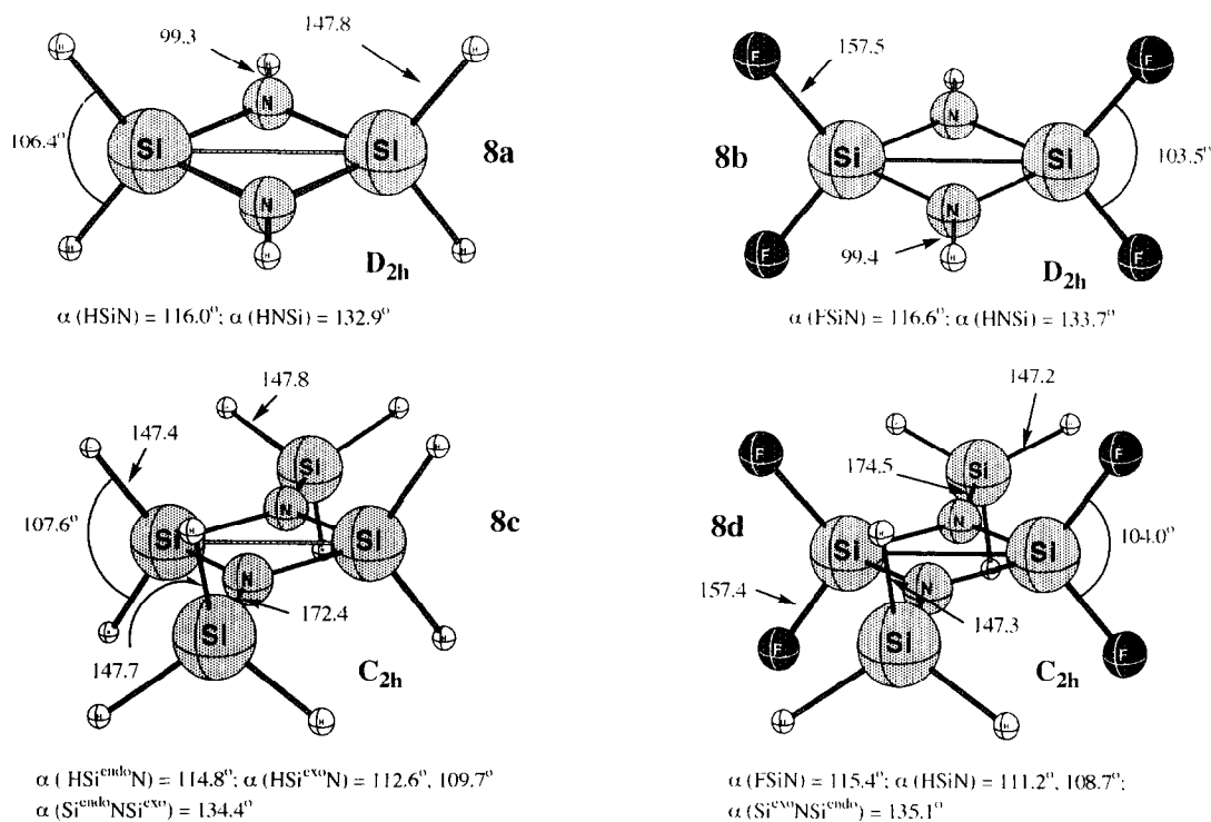
Fig. 2. Calculated geometries of 8a–8d at HF/6-31G* (bond lengths in pm, bond angles in degrees). The geometrical parameters of the inner (SiNSiN) ring are given in Table 4.
