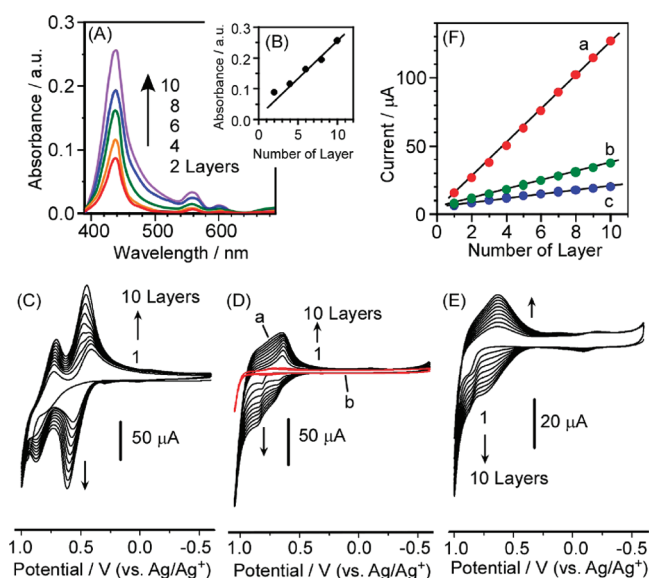
Figure 2. (A) UV–vis spectra and (B) absorbance at 438 nm for PZ4C ECC–LbL films. (C–E) Cyclic voltammograms of (C) PZ4C ; (D) (a) C 60 2C and (b) C 60 1C ; and (E) F4C ECC–LbL films. (F) Layer number dependence of the reduction current of dicarbazole (at 0.45 – 0.6 V) for ECC–LbL films: (a) PZ4C ; (b) F4C ; (c) C 60 2C .
