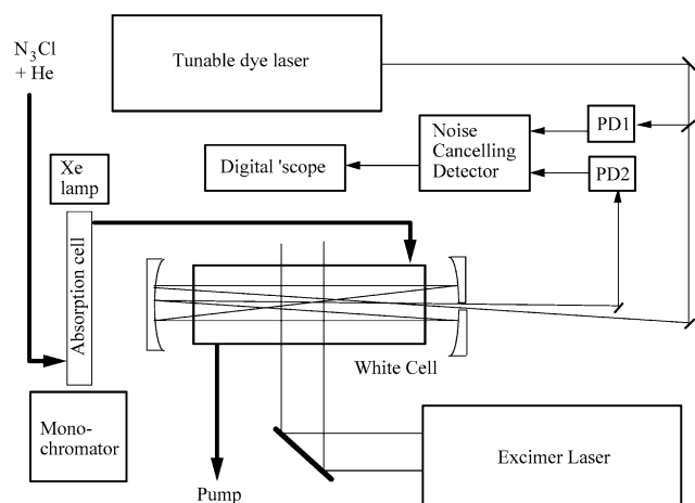
Figure 2. Apparatus used to observe the \text{NCl } b\text{-}X absorption bands. The detection equipment is shown in the configuration used to observe the time dependence of the absorption signal. To record spectra the output from the NCD was processed by a boxcar integrator.
