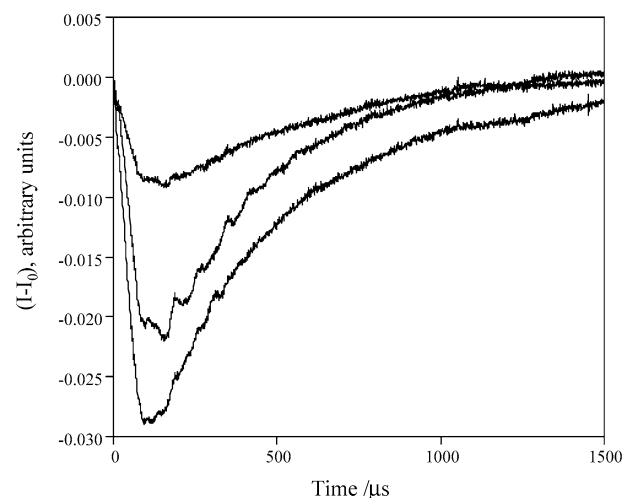
Figure 8. Transient \text{NCl}(X) absorption signals obtained by photolysis of \text{ClN}_3 in the presence of \text{O}_2 . These traces were recorded by monitoring the absorption of the \text{QP}(14) line. They correspond to \text{O}_2 densities of 0 , 8.4 \times 10^{15} and 1.9 \times 10^{16}\ \text{cm}^{-3} . The amplitude of the absorption increases with increasing [\text{O}_2] .
