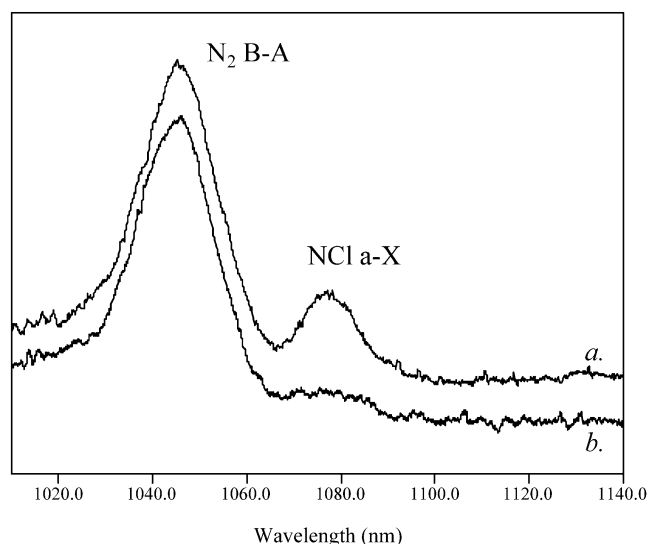
Figure 3. Emission spectra resulting from UV photolysis of \text{ClN}_3 . a. Photolysis at 248 nm. b. Photolysis at 193 nm.
