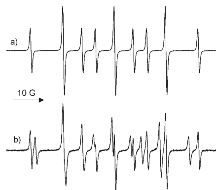
Figure 1. EPR spectra of 1 at 298 K recorded in water a) in the absence and b) in the presence of CB7 (7.0 mM).
