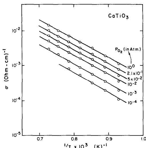
FIG. 9. Temperature dependence of the conductivity of polycrystalline \text{CaTiO}_3 , in the p-type region.
