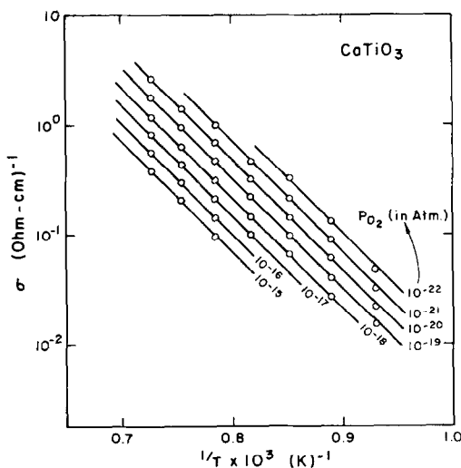
FIG. 3. Temperature dependence of electrical conductivity in polycrystalline CaTiO_3 in the P_{O_2} region 10^{-22} – 10^{-18} atm.
