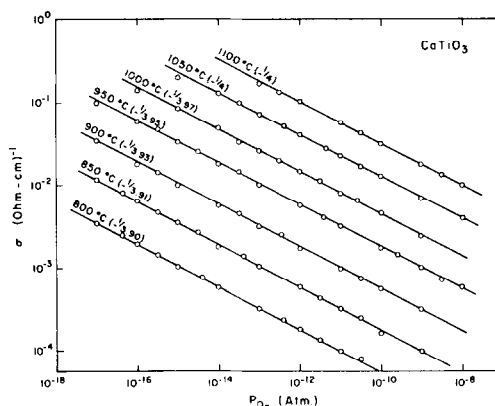
FIG. 4. The electrical conductivity of polycrystalline \text{CaTiO}_3 as a function of oxygen partial pressure at constant temperature, from 10^{-17} to 10^{-8} atm.
