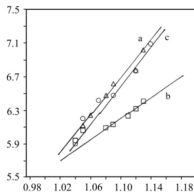
Fig. 4 Linearisation curves for step II of a – (\text{C}_6\text{H}_5\text{CH}_2)_3\text{Sn}(\text{L}^2) ; b – (\text{C}_6\text{H}_5\text{CH}_2)_2\text{Sn}(\text{L}^2)_2 ; c – (p\text{-ClC}_6\text{H}_4\text{CH}_2)_3\text{Sn}(\text{L}^2)
