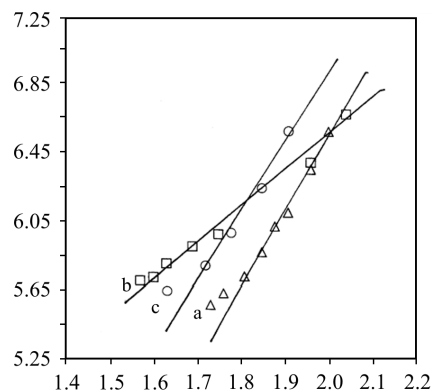
Fig. 3 Linearisation curves for step I of a – (\text{C}_6\text{H}_5\text{CH}_2)_3\text{Sn}(\text{L}^2) ; b – (\text{C}_6\text{H}_5\text{CH}_2)_2\text{Sn}(\text{L}^2)_2 ; c – (p\text{-ClC}_6\text{H}_4\text{CH}_2)_3\text{Sn}(\text{L}^2)
