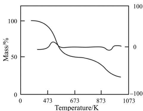
Fig. 5 TG and DTA curves of (\text{C}_6\text{H}_5\text{CH}_2)_3\text{Sn}(\text{L}^1) complex
