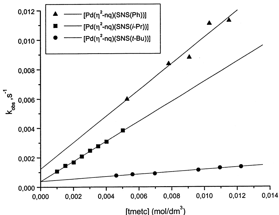
Fig. 1. Fit of k_{\text{obs}} values to added tmctc concentration for the reaction [\text{Pd}(\eta^2\text{-nq})(\text{SNS}(\text{R}))] + \text{tmctc} = [\text{Pd}(\eta^2\text{-tmctc})(\text{SNS}(\text{R}))] + \text{nq} ( \text{R} = i\text{-Pr} , t\text{-Bu} , \text{Ph} ) (Eq. (1)).
