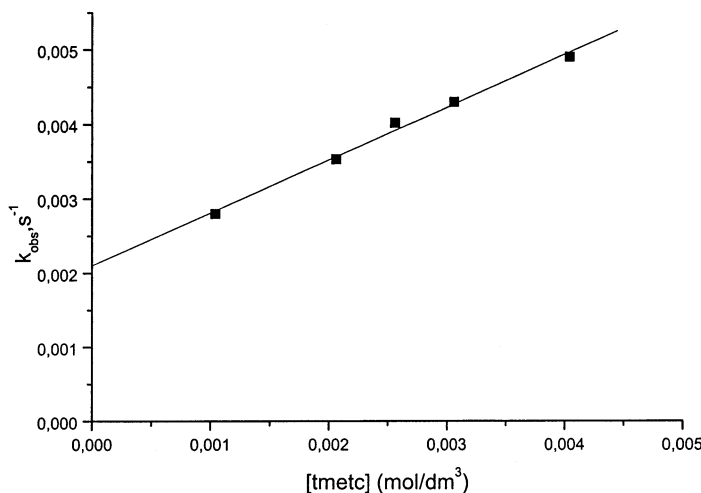
Fig. 3. Fit of k_{\text{obs}} to added tmctc concentration under pseudo-first order conditions for both direct and reverse paths of reaction (3).
